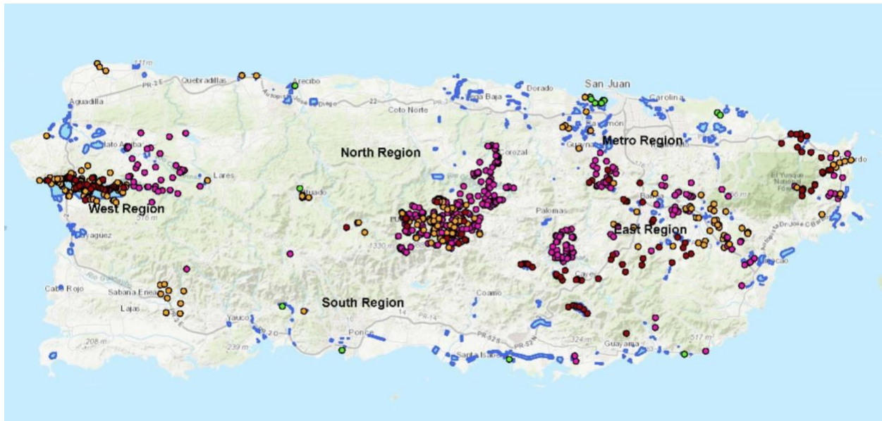
Figure 70. Stormwater System Damages due to Hurricane María 171
